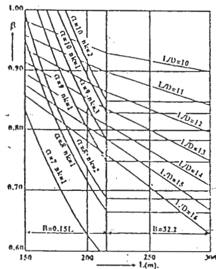
Figure (3) B Versus LBP at Constant L/D, R_C and N_{CH} , [18].
