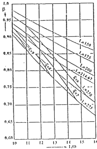
Figure (4) B Versus L/D at Constant LBP and S_C , [18].
