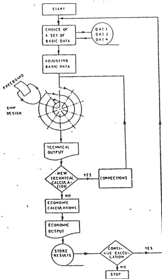
Figure (8) Schematic Representation of PROCAL Subsystem, [19].
