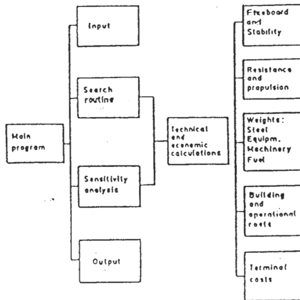
Figure ( 9 ) Schematic Representation of FLEET Subsystem, [19].
