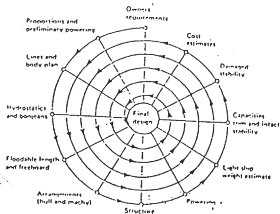
Figure ( 1 ) Design Spiral for All Merchant Ships, [10].
